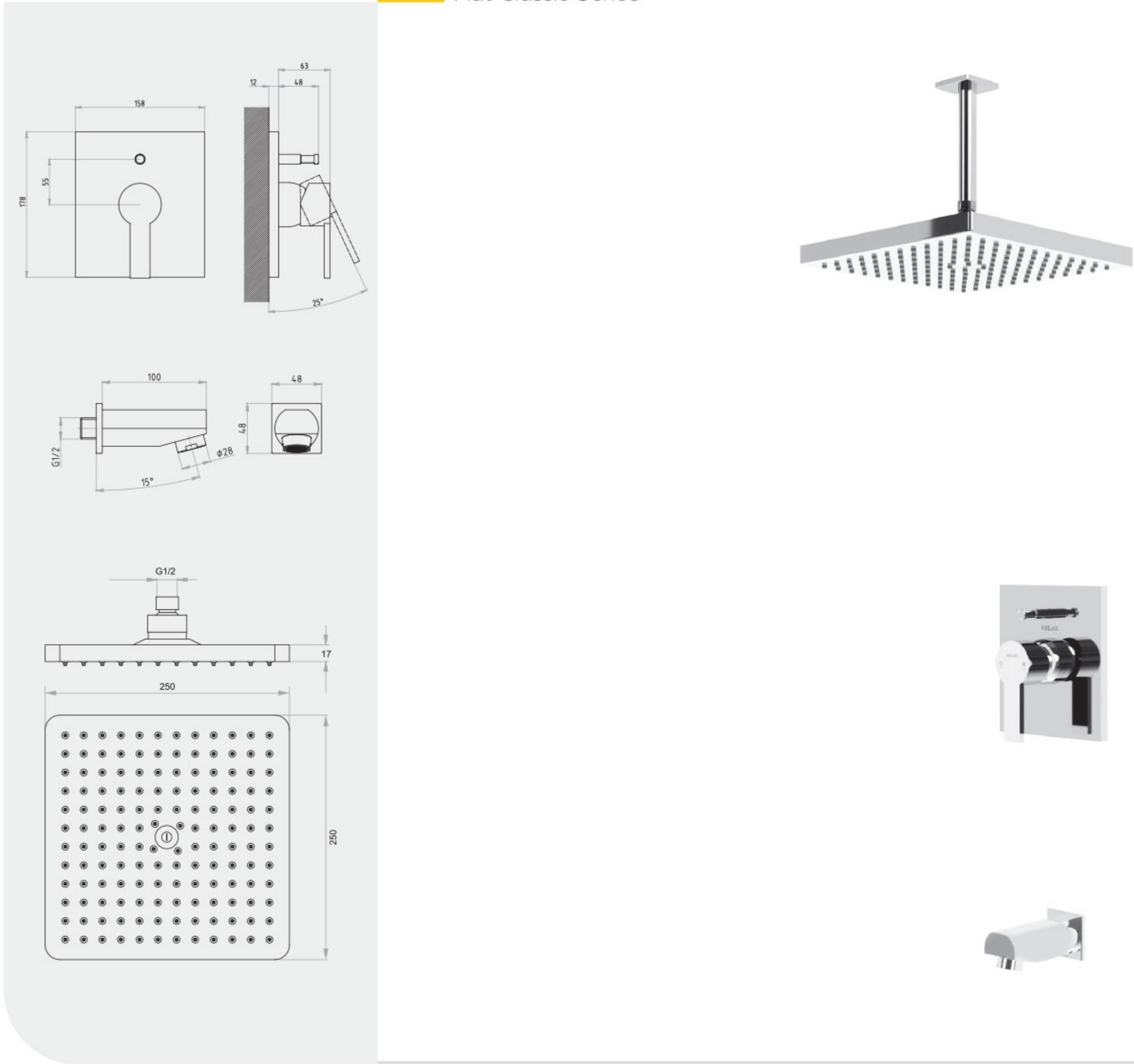
Shower Set, type 2 Flat Classic Series
