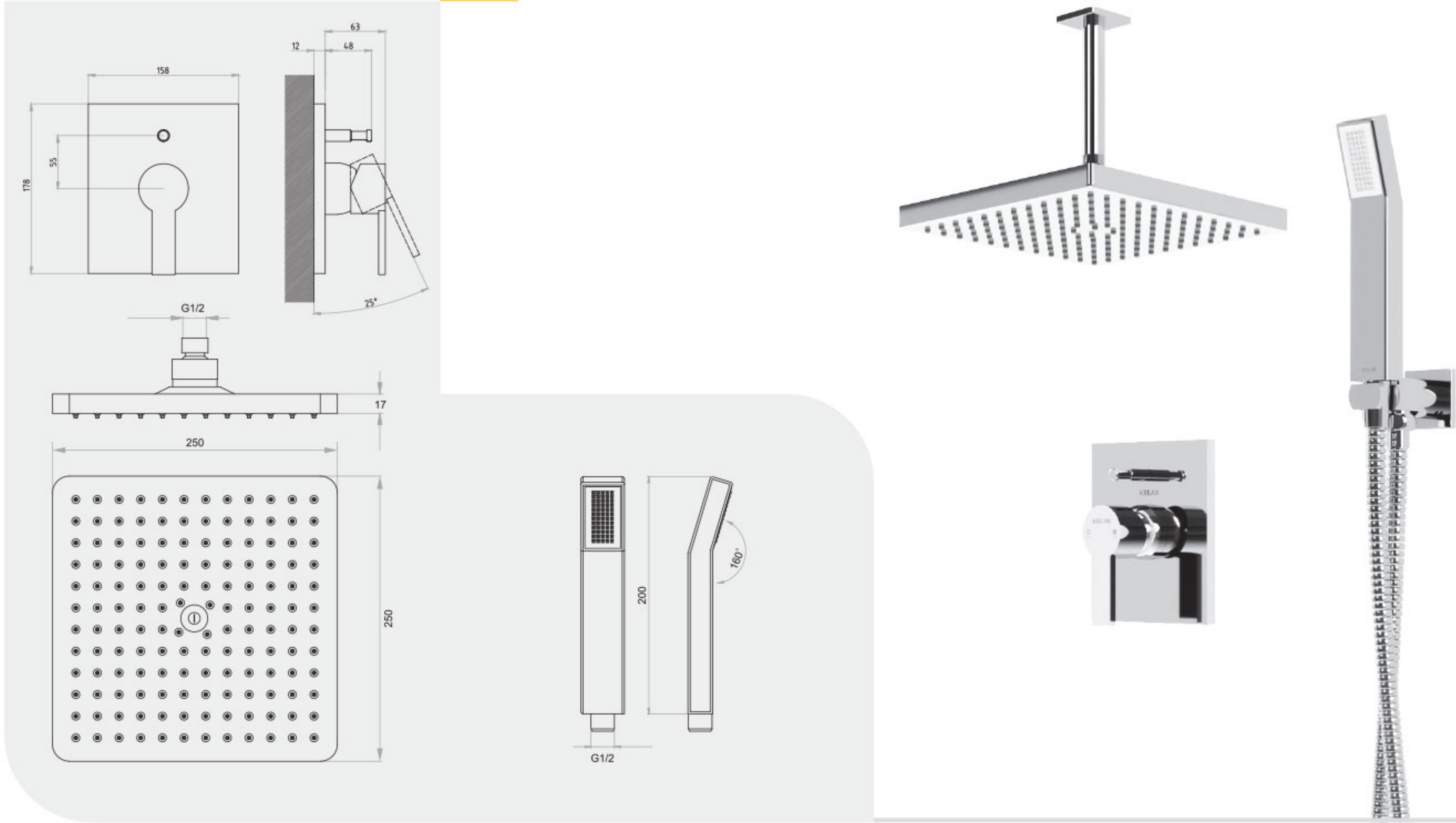
Shower Set, type 3 Flat Classic Series
